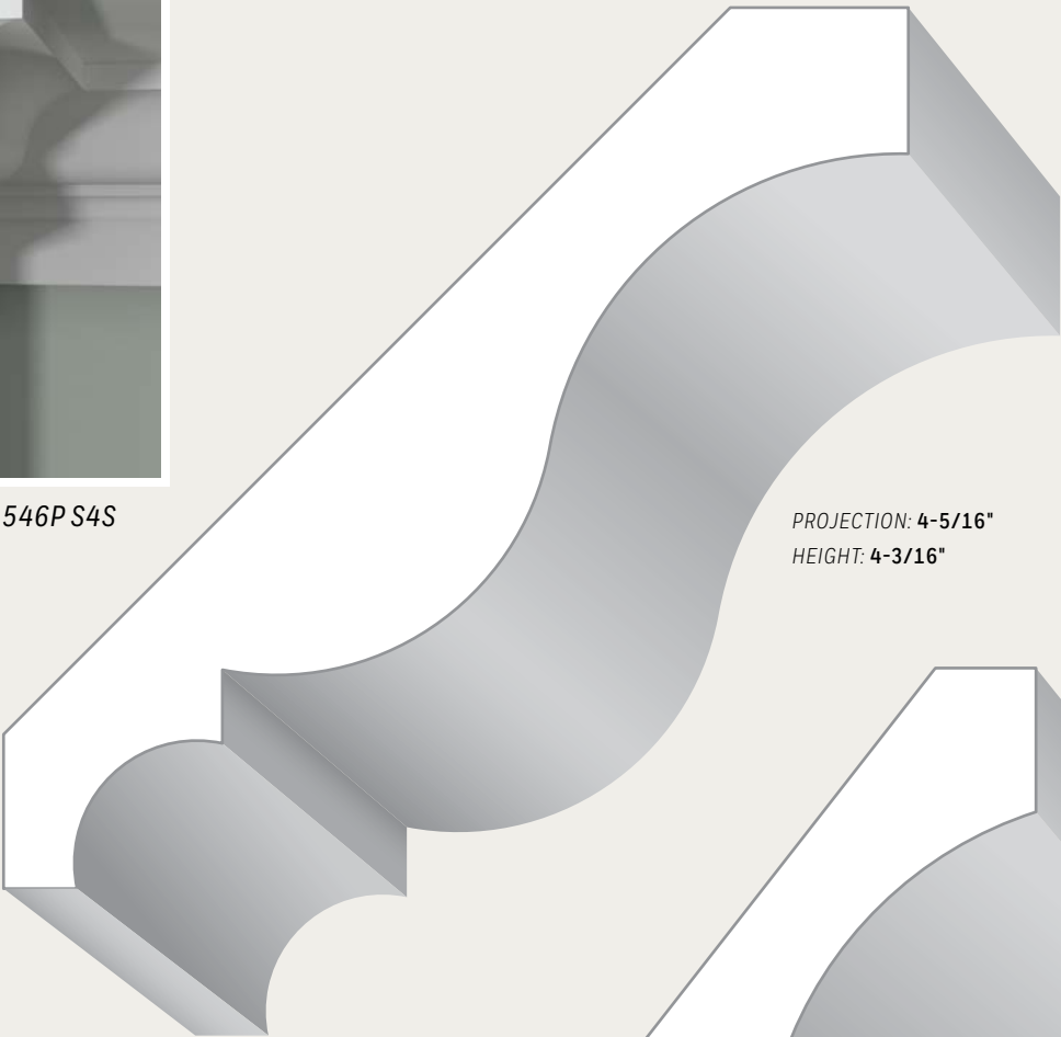
6" Net Heavy Crown Moulding with Cove
