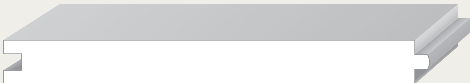
1 x 8 T&G Center Match
