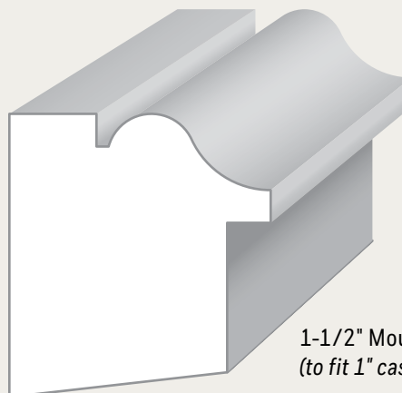
SL112MBP Backband with SL4BWCP Casing
