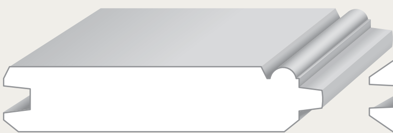
1 x 4 T&G Beaded 1 Edge Ceiling (Small V)
