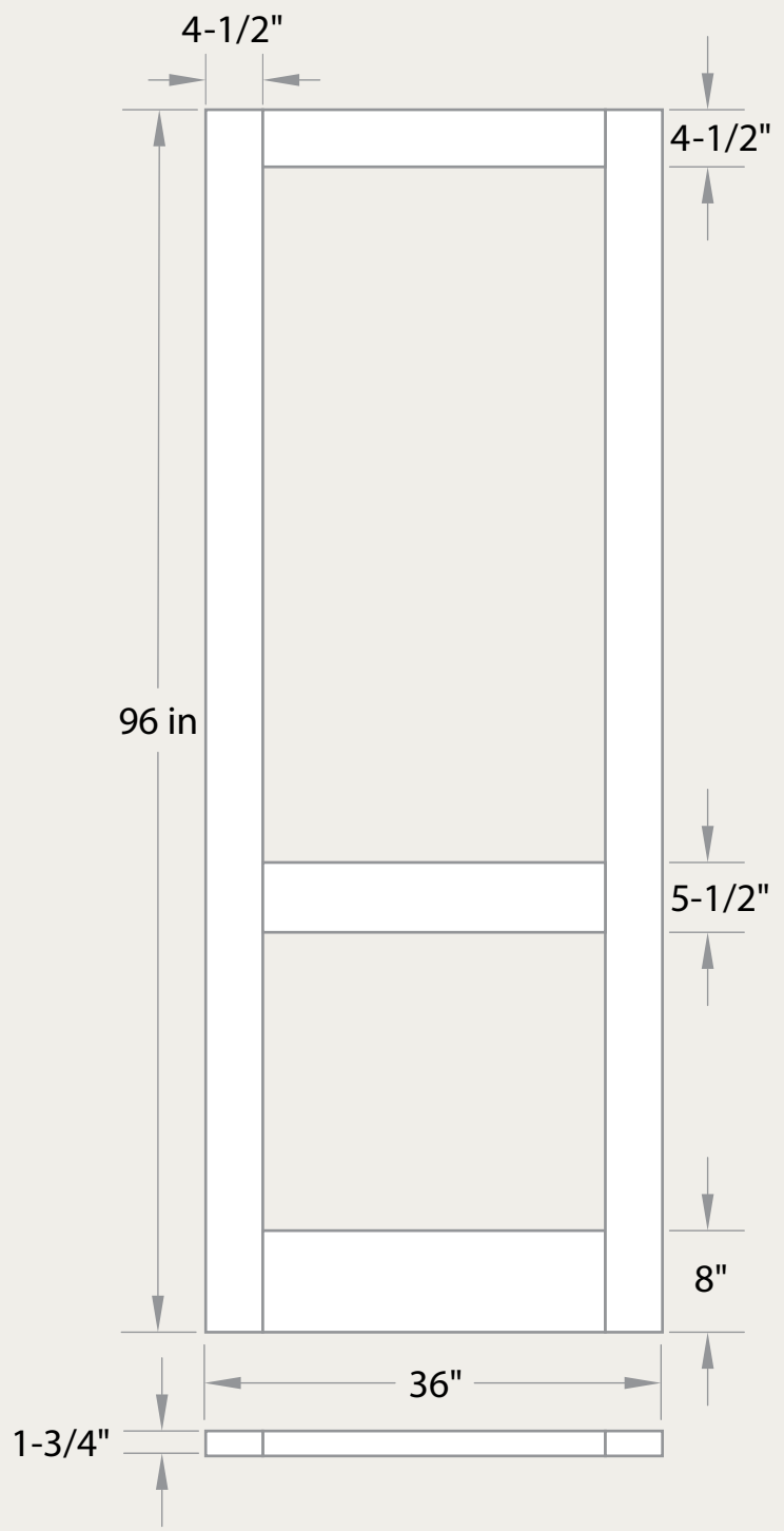
3/0 x 6/8 x 1-3/4 2 Section Screen Door w/ Spline dado (screen & spline not included, dado 3/8 x 3/4")
