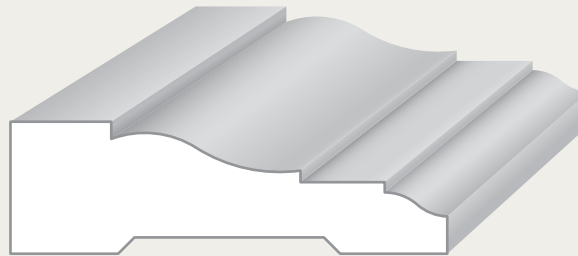
1 1/16" x 2-1/4" Moulded Casing
