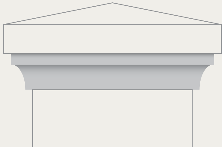
Pyramid Post Cap Base (fits 5-1/2" net x 5-1/2" net posts)
