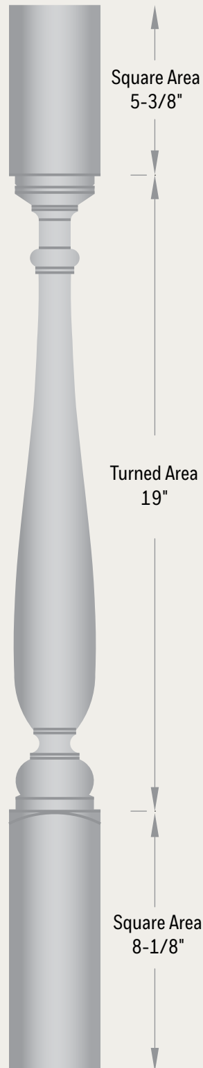
TREATED PINE *234TB32 Square Top Colonial – 2-3/4" x 32"
