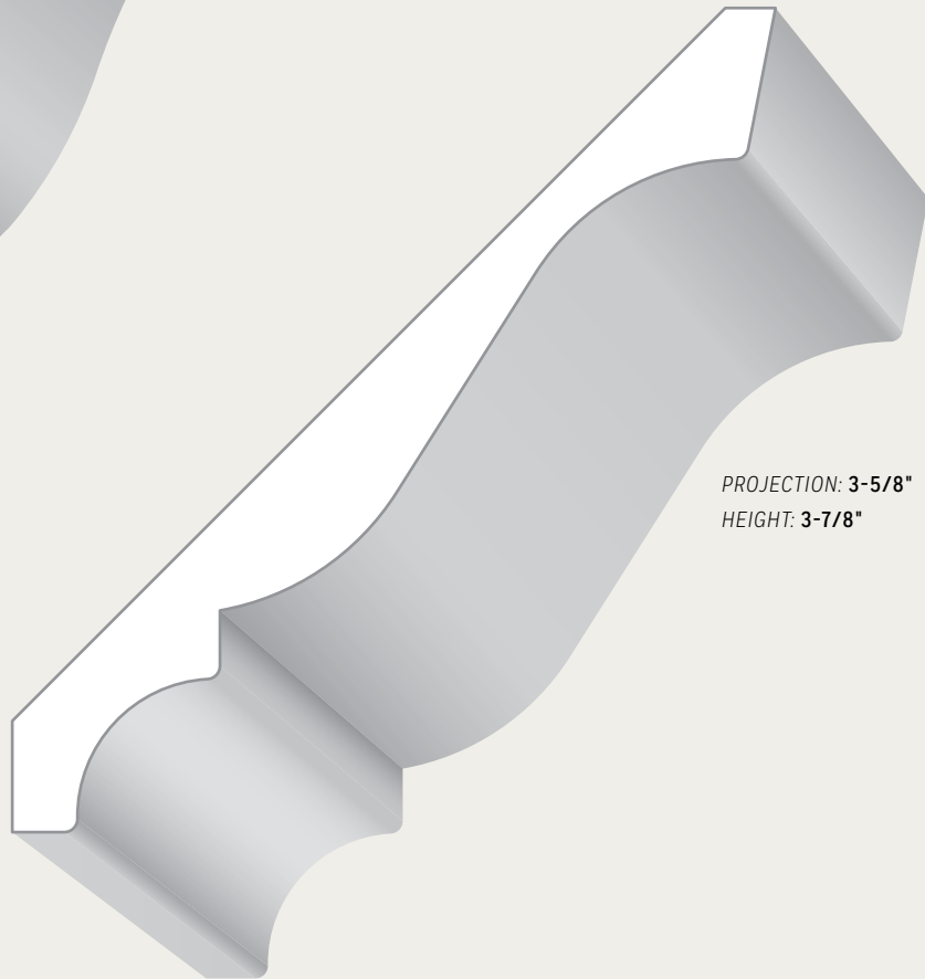
5-1/4" MDF Crown Moulding with Cove – 16'
