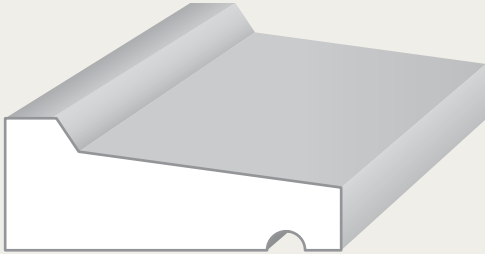
11/16" x 1-3/4" Drip Cap
