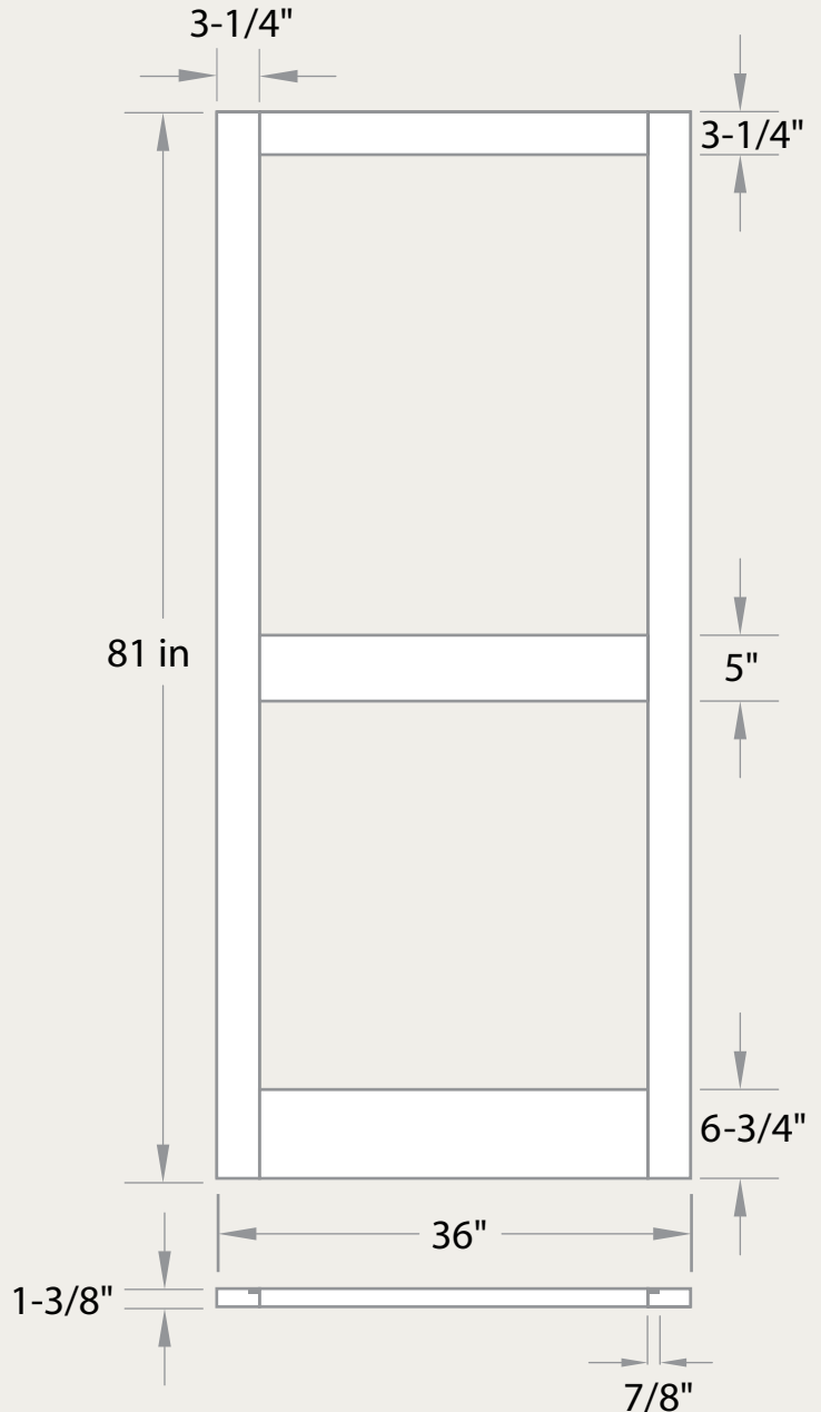
3-0 x 6-9 Treated Screen Door Plain, 1-3/8" Screen included
