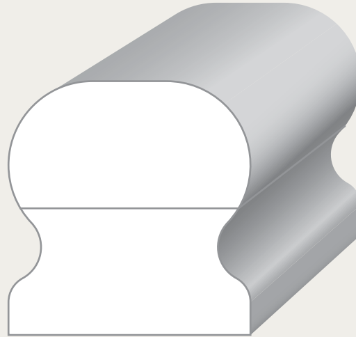
2" Exterior Stair Rail (net dimensions: 1-13/16" x 1-7/8")
