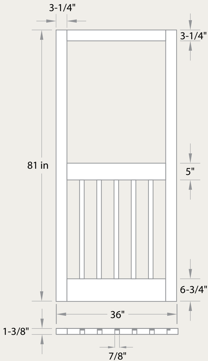
3-0 X 6-9 Treated Screen Door 5 Bar, 1-3/8" Screen included
