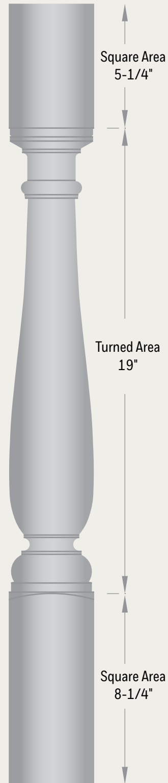
TREATED PINE *312TB32 Square Top Colonial – 3-1/2" x 32"
