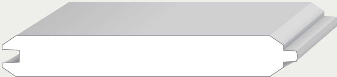
1 x 6 T&G V-Edge (Large V)
