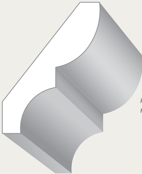
2-3/4" Bed Moulding
