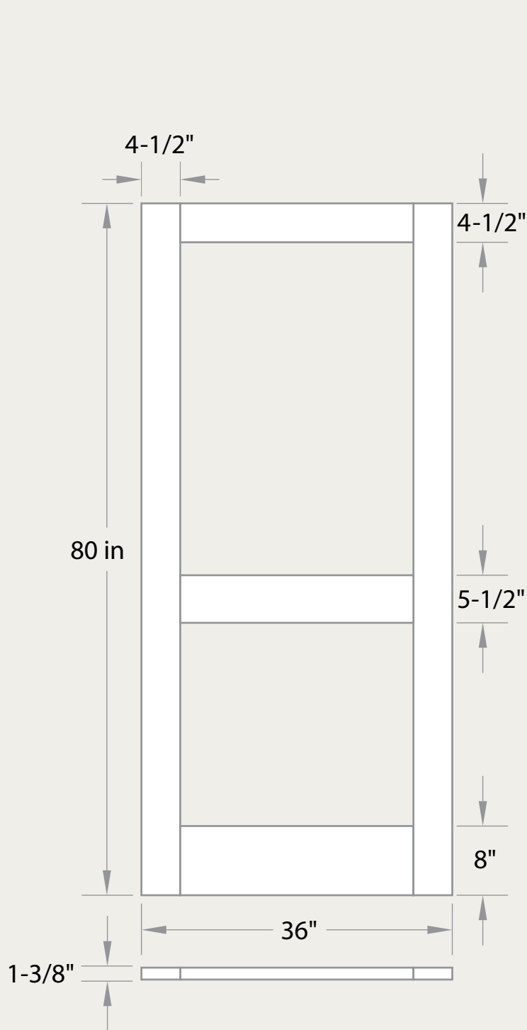
3/0 x 6/8 x 1-3/8 2 Section Screen Door w/ Spline dado (screen & spline not included, dado 3/8 x 3/4")
