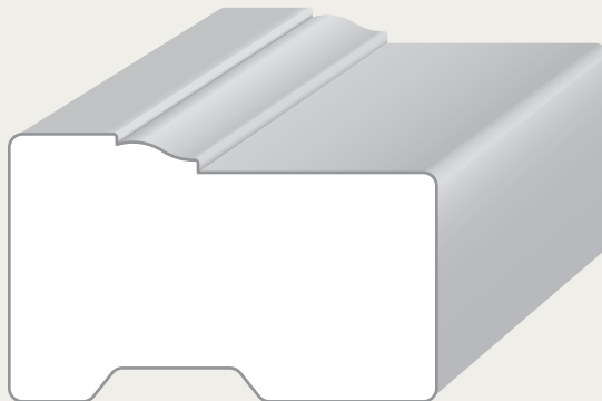
1-1/4" x 2" Brick Moulding
