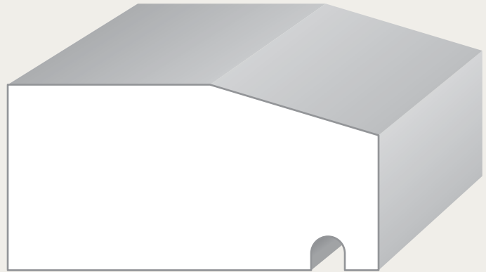
1-3/8" x 2-3/4" Drip Cap*
