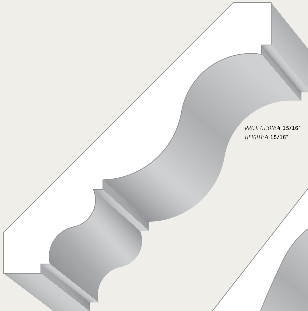
6-7/8" Multi Look Crown Moulding
