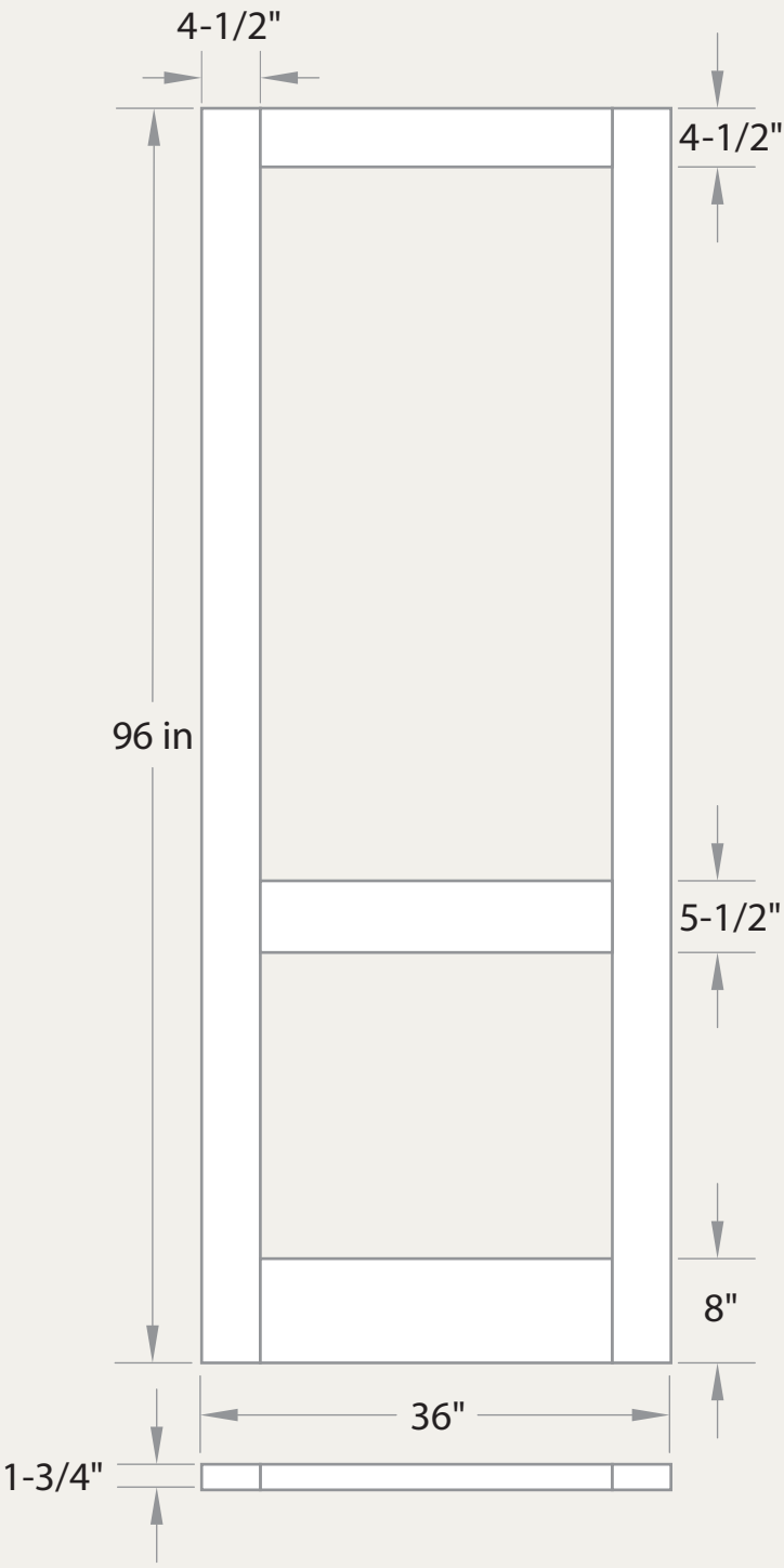
3/0 x 6/8 x 1-3/4 2 Section Screen Door w/ Spline dado (screen & spline not included, dado 3/8 x 3/4")
