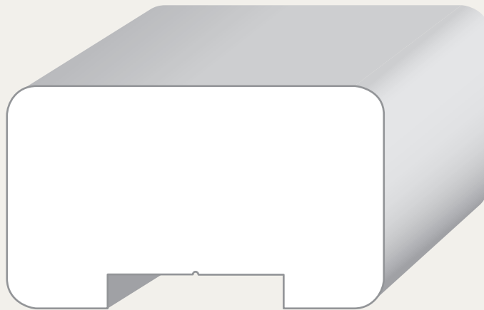
6000 1-5/8" x 2-3/4" Solid Cap Handrail Plowed for 1-1/4" Baluster
