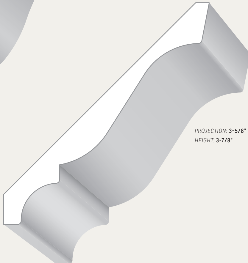
5-1/4" MDF Crown Moulding with Cove – 16'
