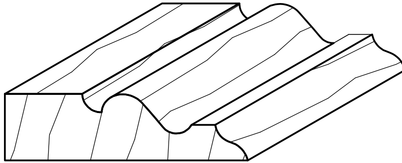
2-1/2" BACK MOULDING (net dimensions: 11/16" X 2-1/2") SL212BM
