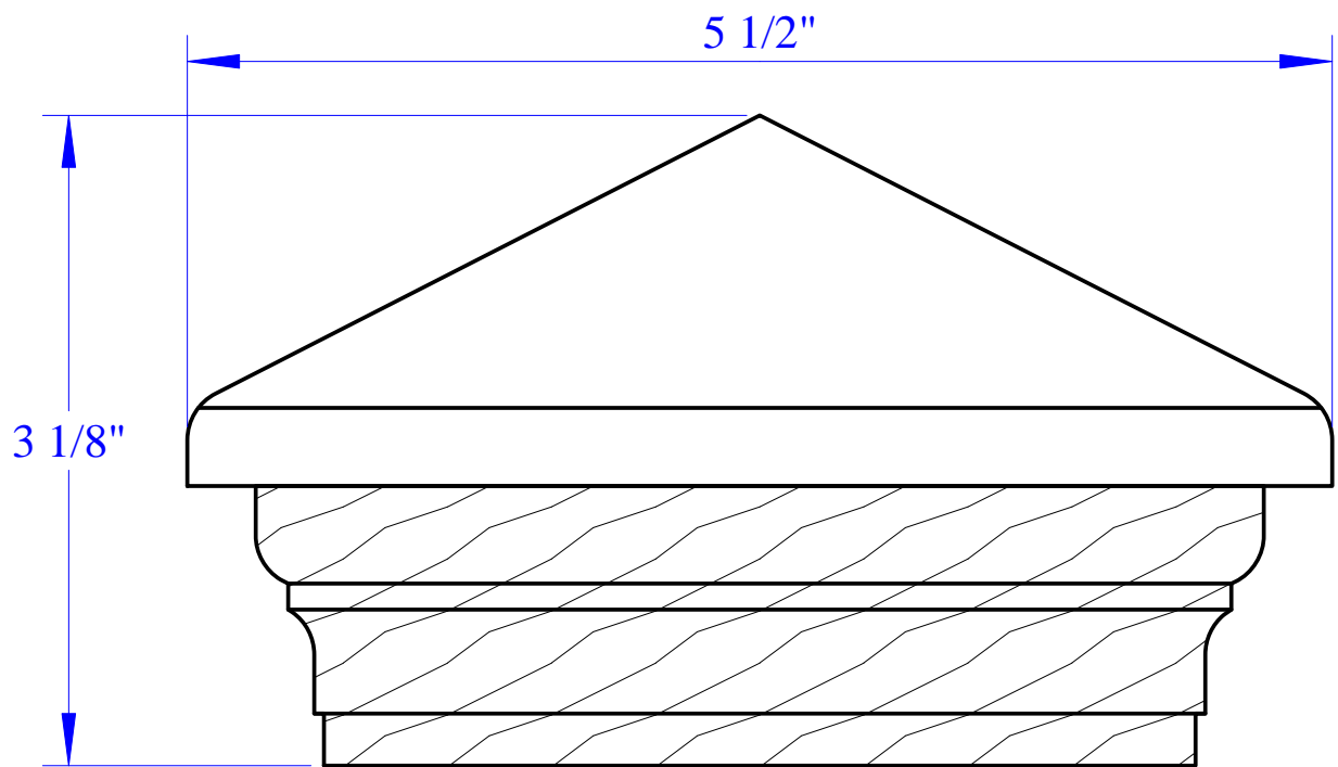
VICTORIA HIGH POINT (fits 3-1/2" net x 3-1/2" net posts) VC1 - copper top with western red cedar trim
