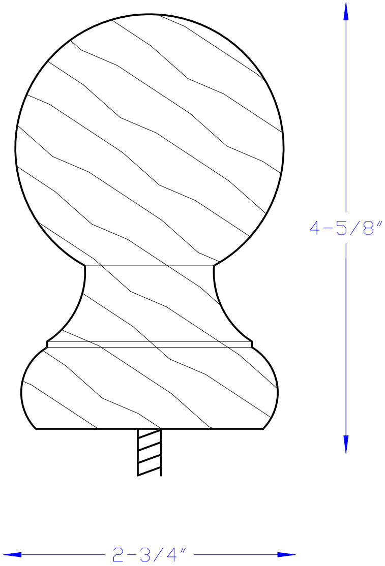
SMALL BALL TOP TBT3 - treated pine
