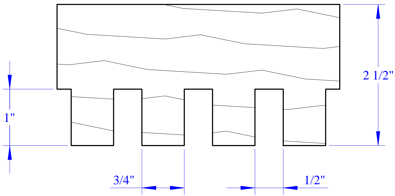
INTERIOR DENTIL MOULDING SLIDMP - poplar
