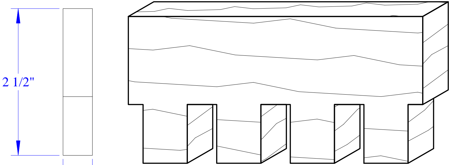
INTERIOR DENTIL MOULDING SLIDMP - poplar
