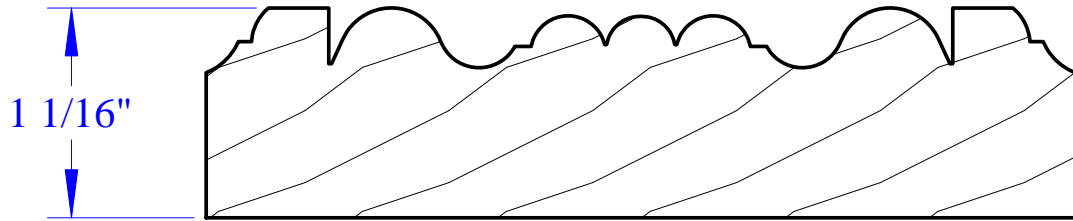
SL6A - 4-1/2" X 4-1/2" ROSETTE
