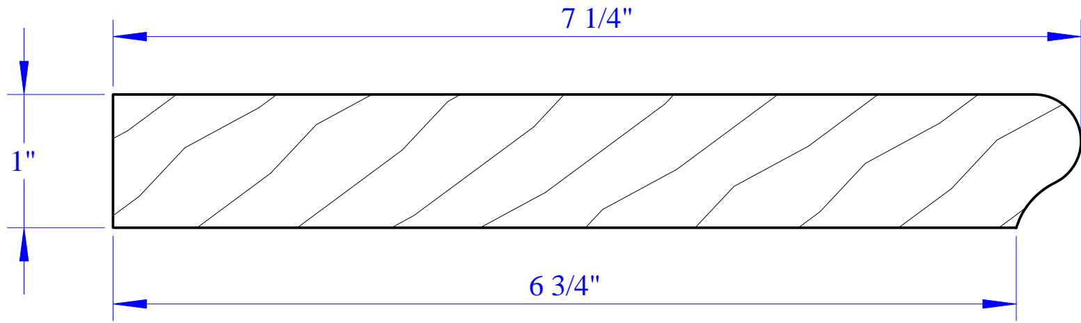
5/4" X 8" WINDOW STOOL SL54WS8P - poplar
