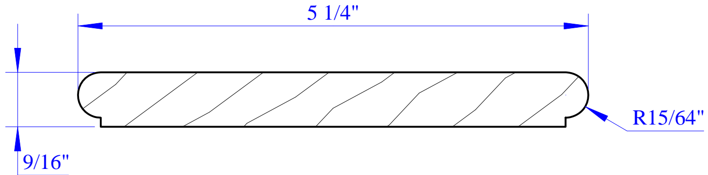
9/16" X 5-1/4" DOUBLE BEADED STOP SL514DB - yellow pine
