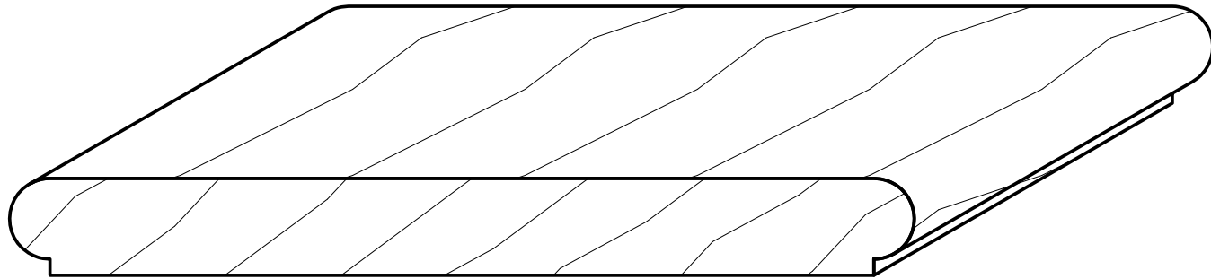
9/16" X 5-1/4" DOUBLE BEADED STOP SL514DB - yellow pine
