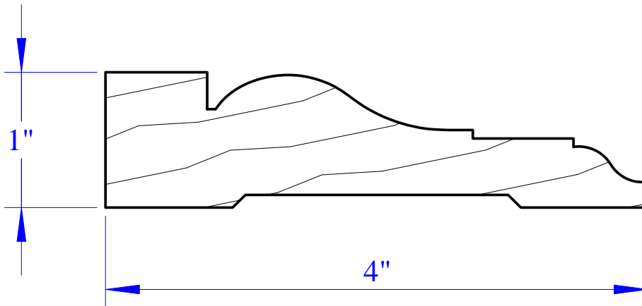
1" X 4" HEAVY MOULDED CASING SL4HMCP - poplar
