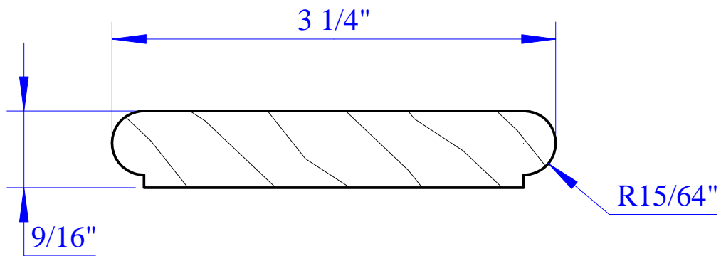
9/16" X 3-1/4" DOUBLE BEADED STOP SL4DB - yellow pine
