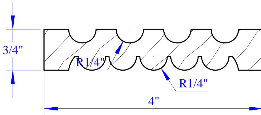
3/4" X 4" NET FLUTED & REEDED CASING SL344NFP - poplar
