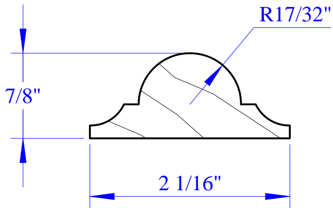
2" CHAIR RAIL LIKE WILLIAMSBURG SL2CRLW - poplar
