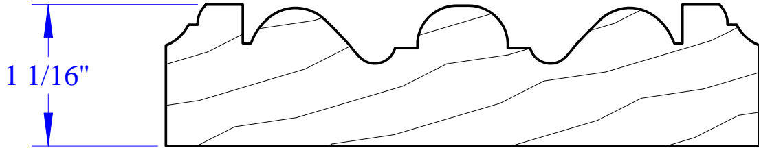
SL13A - 4-1/2" X 4-1/2" ROSETTE
