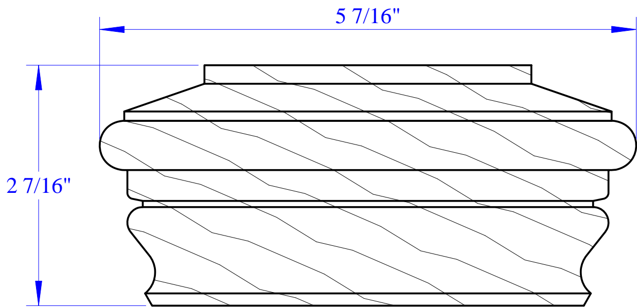
NEWPORT CLASSIC (fits 3-1/2" net x 3-1/2" net posts) NC2 - western red cedar
