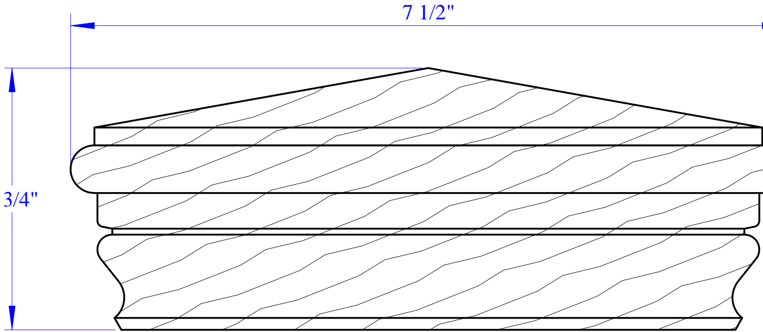
NEWPORT HIGH PYRAMID (fits 5-1/2" net x 5-1/2" net posts) NC1E - western red cedar
