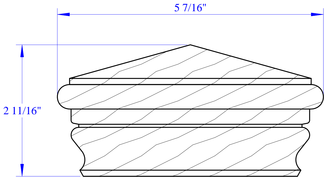
NEWPORT HIGH PYRAMID (fits 3-1/2" net x 3-1/2" net posts) NC1 - western red cedar
