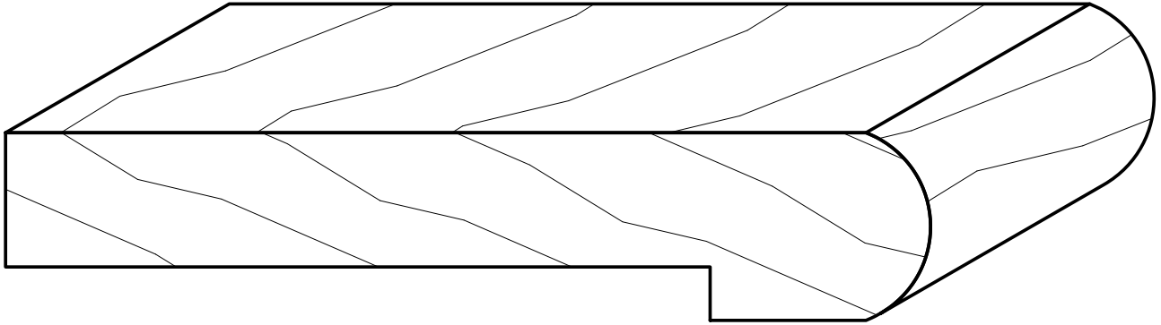
5-1/4" LANDING TREAD 80905 - red oak
