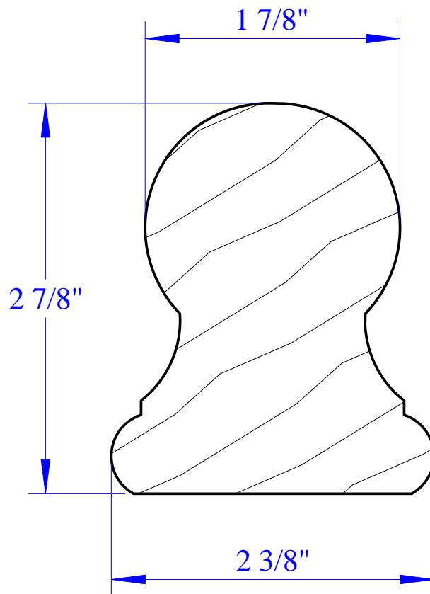
2-3/8" X 2-7/8" PROFILE 6109 STAIR RAIL 6109_ - variety of species available
