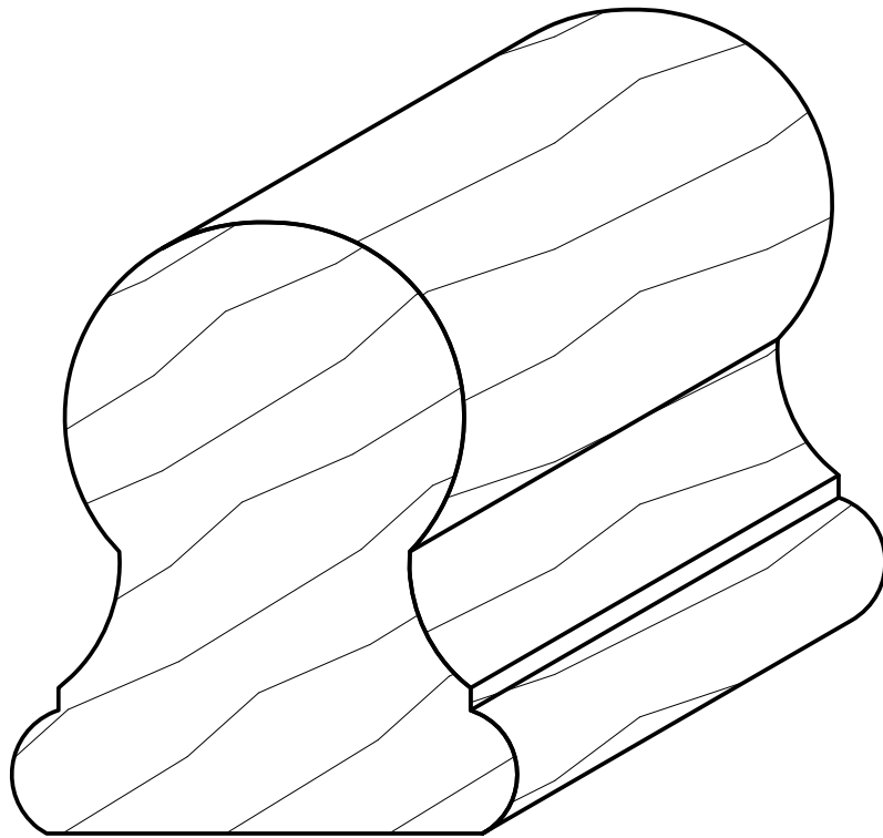
2-3/8" X 2-7/8" PROFILE 6109 STAIR RAIL 6109_ - variety of species available
